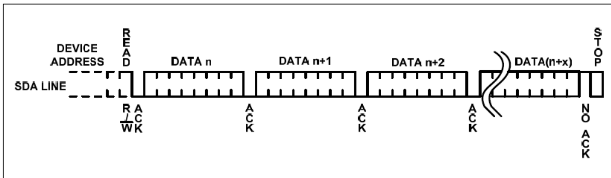
Figure 12 · Sequential Read
